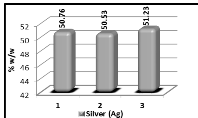
Graphical Representation of Silver Content in Taragarbha Pottali (Batch to Batch Consistency) by ICP-OES
