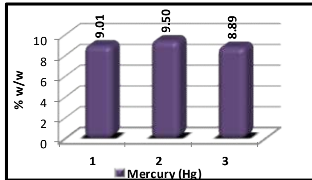
Graphical Representation of Mercury Content in Taragarbha Pottali (Batch to Batch Consistency) by ICP-OES
