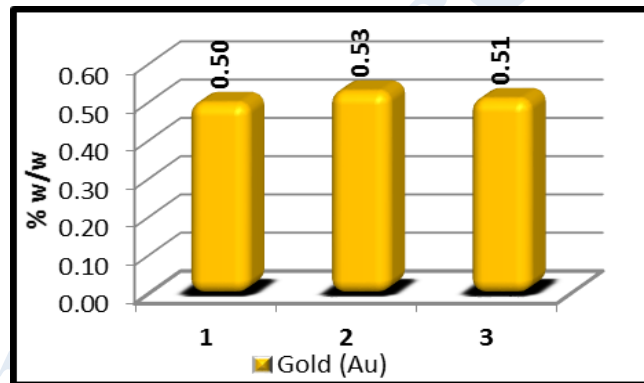
Graphical Representation of Gold Content in Taragarbha Pottali (Batch to Batch Consistency) by ICP-OES
