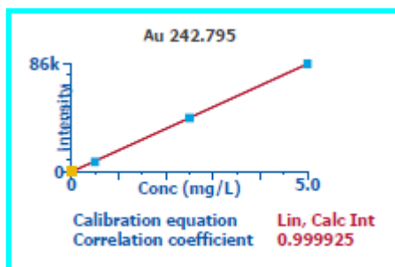
Standard Linear Graph of Au prepared in correlation with NIST Traceable Reference Standard
