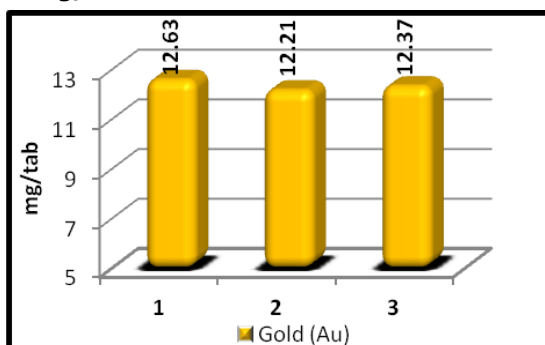
Graphical Representation of Gold Content in Suvarna (Svarna) Bhasma Tablet (Batch to Batch Consistency) by ICP-OES
