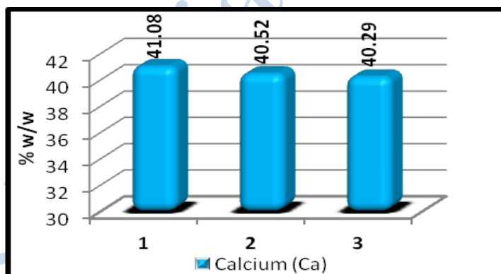
Graphical Representation of Calcium Content in Shouktik (Muktashukti) Bhasma (Batch to Batch Consistency) by ICP-OES
