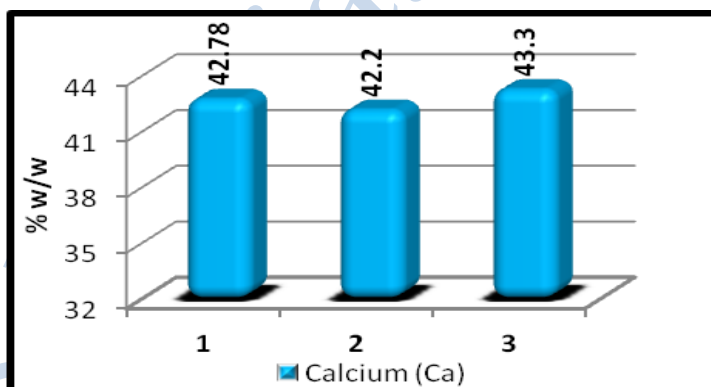
Graphical Representation of Calcium Content in Mouktik (Mukta) Bhasma (Batch to Batch Consistency) by ICP-OES
