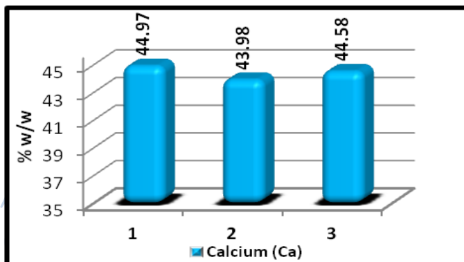
Graphical Representation of Calcium Content in Kukkutandatvak Bhasma (Batch to Batch Consistency) by ICP-OES
