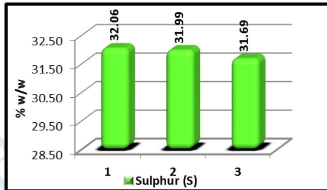
Graphical Representation of Sulphur Content in Hemagarbha Pottali (Batch to Batch Consistency) by ICP-OES
