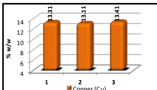
Graphical Representation of Copper Content in Hemagarbha Pottali (Batch to Batch Consistency) by ICP-OES
