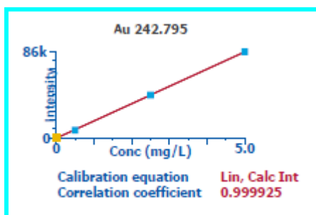
Graphical Representation of Gold Content in Brahmi Vati Suvarnayukta (Batch to Batch Consistency) by ICP-OES
