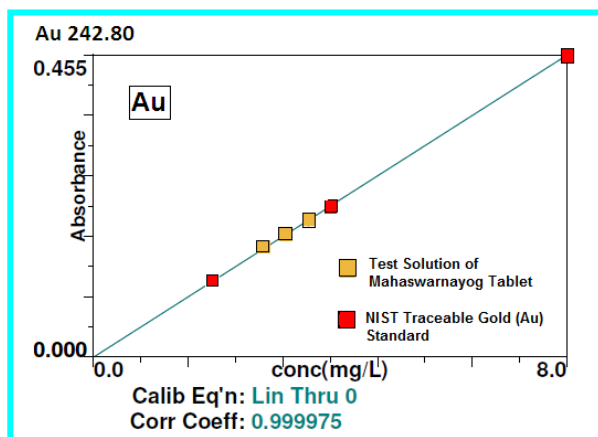
Standard Linear Graph of Au prepared in correlation with NIST Traceable Reference Standard
